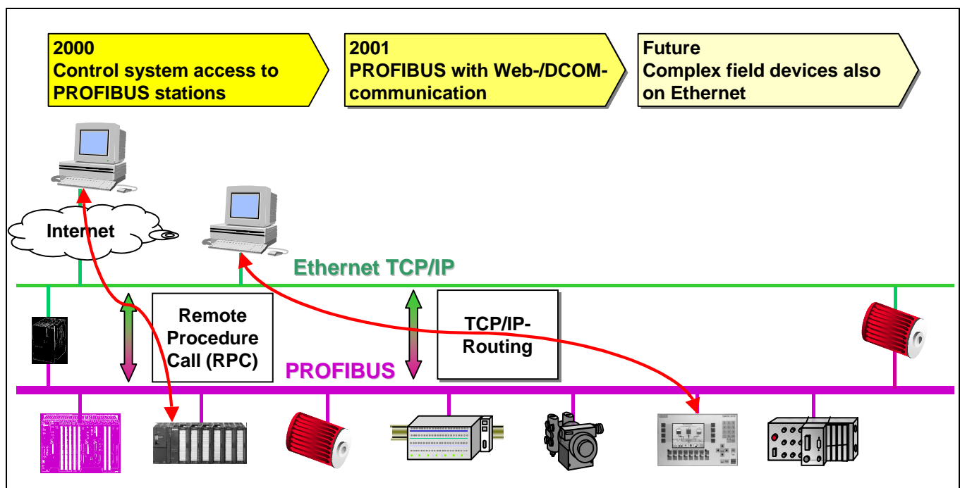
Fig.23: Integration of Ethernet in the communication with PROFIBUS
