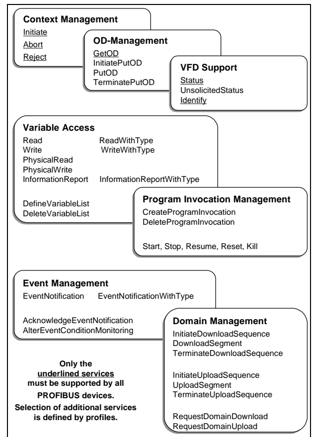
Fig. 14: Overview of FMS services
